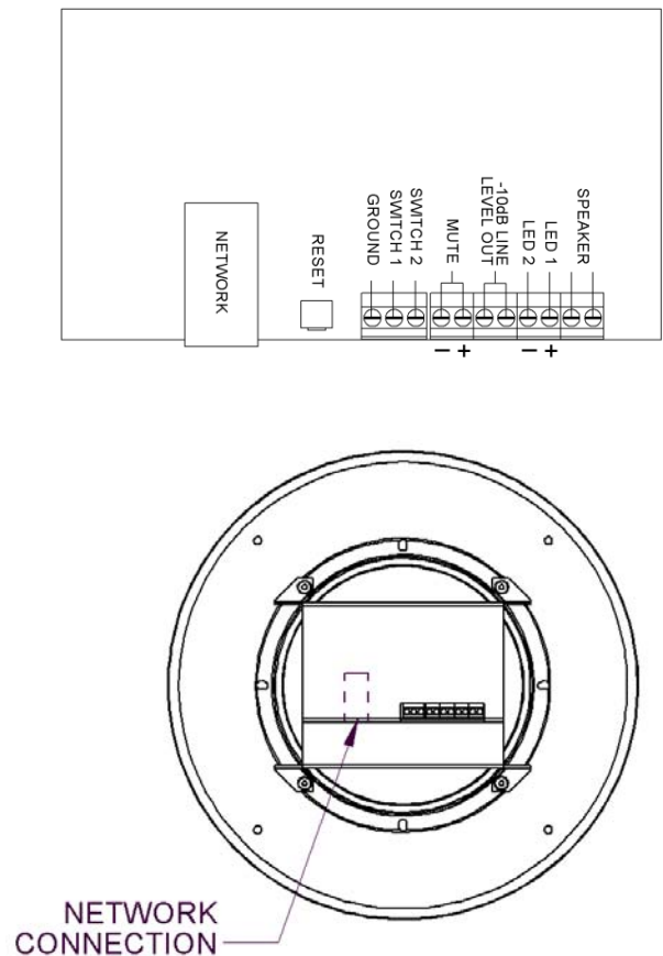
Figure 1. VIP-120A Connections
